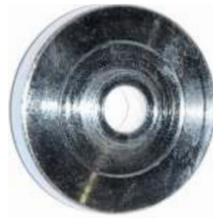
Втулка (Bushing Forged) CLAAS: COMMANDOR, DOMINATOR, MEDION, MEGA Артикул (Article): 061196.U10
